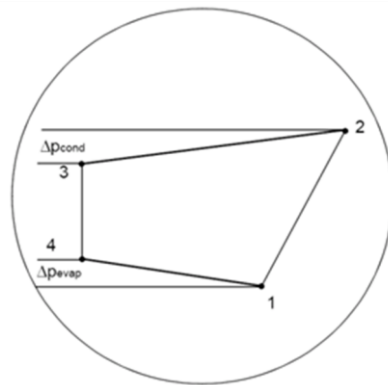
Figure 18. Pressure drops in evaporator and condenser.
