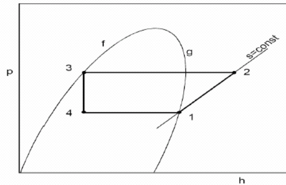
Figure 14. Refrigeration cycle.
