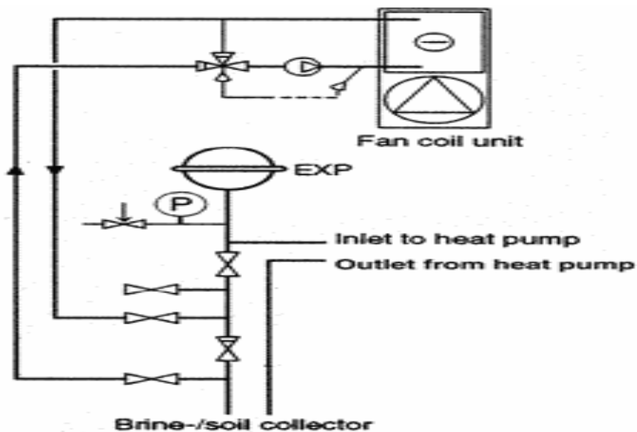
Figure 3. Diagram of cooling system.
