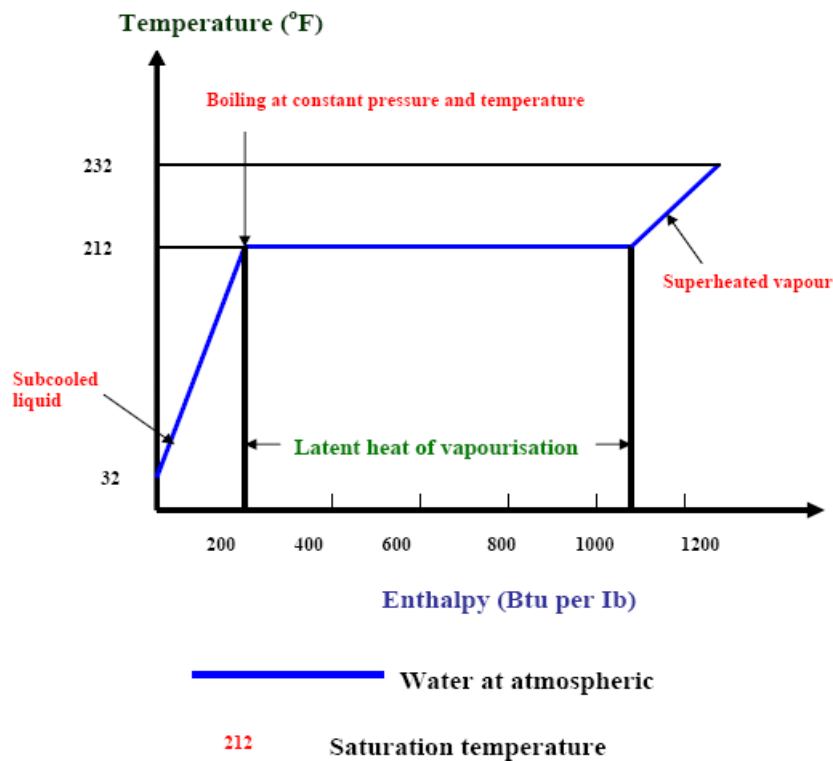
Figure 13. Water undergoing a change of state.
