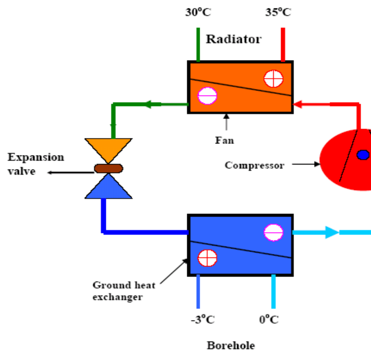
Figure 2. Detail of the GSHP circuit.
