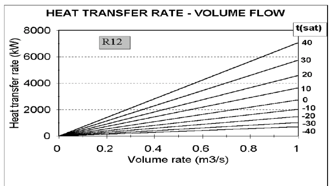
Figure 5. Heat transfer rate versus volume rate.
