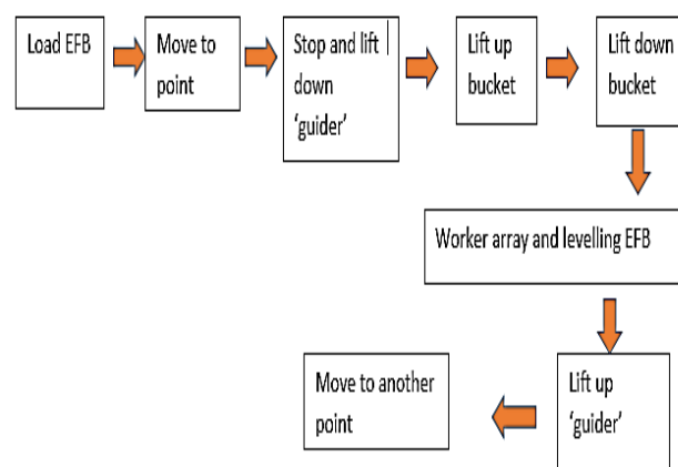
Figure 7: Process Flow Diagram of EFBM motion study
